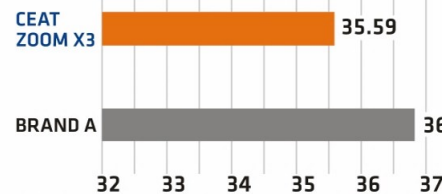
DRY BRAKING DISTANCE (In Meters)
