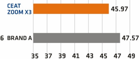
WET BRAKING DISTANCE (In Meters)
